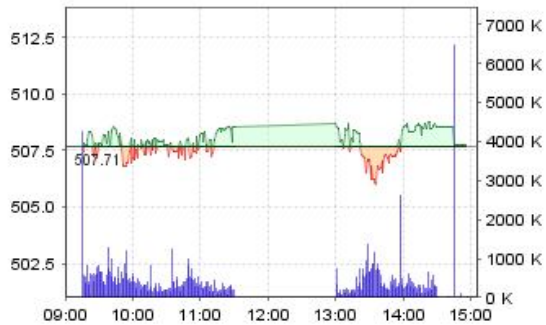
VN-Index
